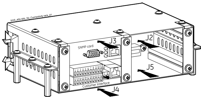
Рис. 9-1 Connectivity rack
